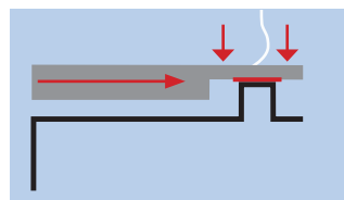
Contactor position for "fittings locked"
