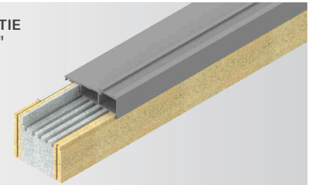
DORPEL ASSORTIMENT THERMOTOP
