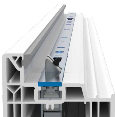
16 mm-Stulp
